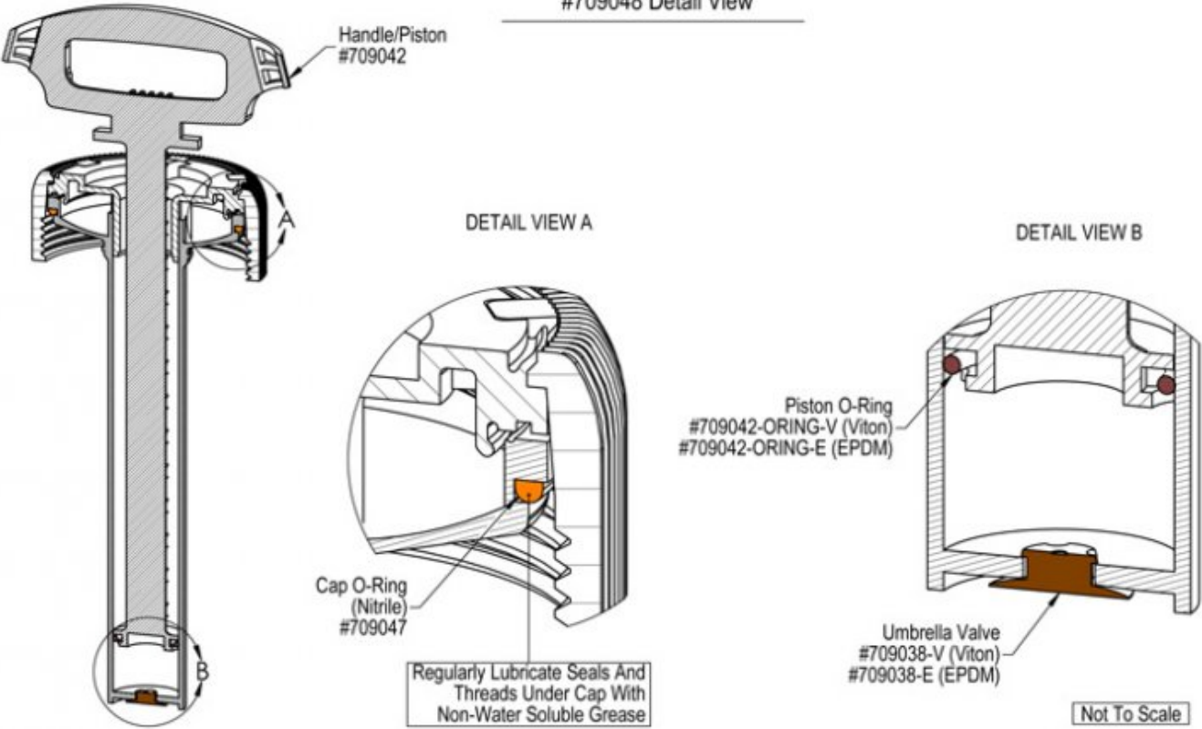
#709048 Detail View
